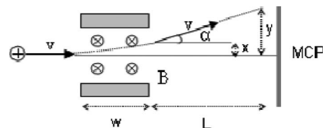
FIG. 5. A schematic presentation of the model used to calculate the deflection y at the MCP position at a distance L behind a perpendicular applied magnetic field B . A positive ion with speed v entering the magnetic field B of length w will exit the field under angle \alpha .
