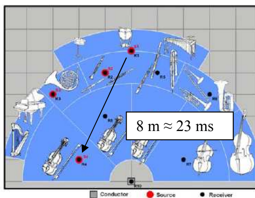
Figure 7: source and receiver position S1R4
