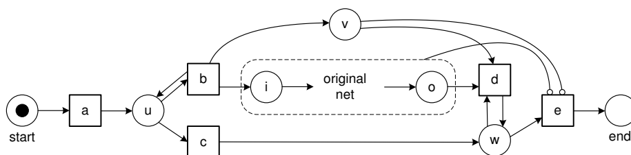
Fig. 14. Construction showing that generalized soundness can be expressed in terms of weak soundness for WF-nets with inhibitor arcs.
