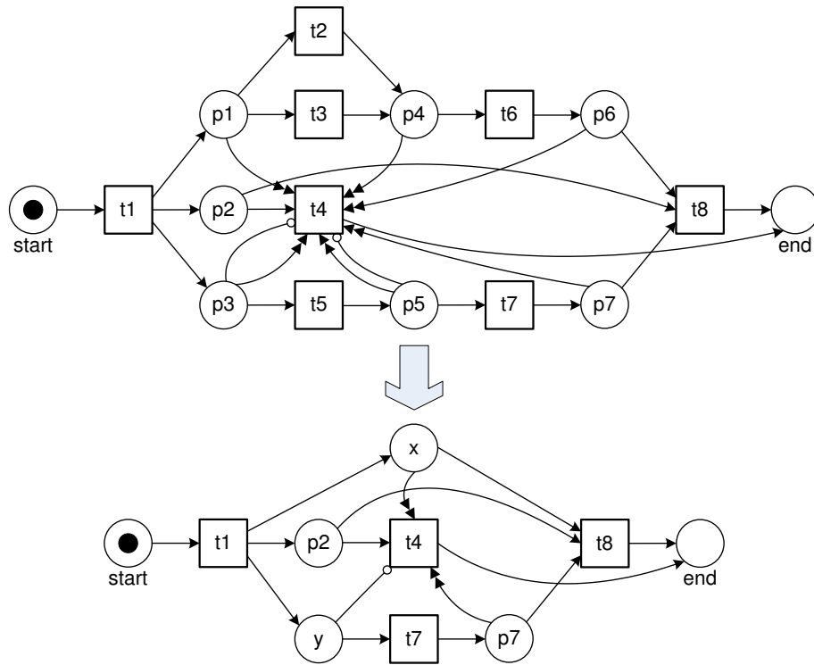
Fig. 23. Partial reduction of a WF-net with reset and inhibitor arcs.
