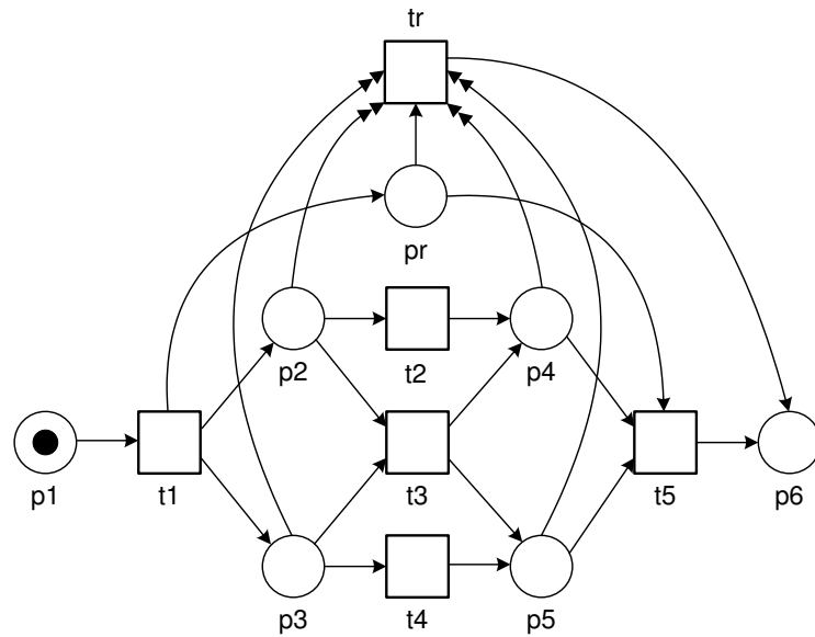
(c) Extended Petri net with reset arcs
