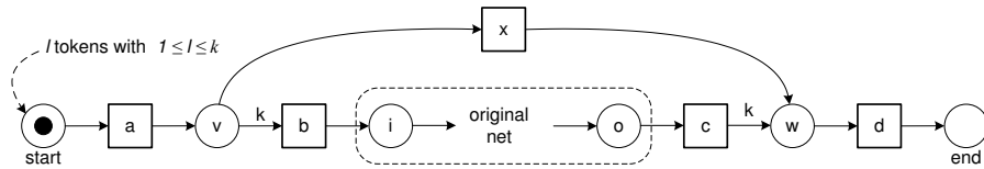
Fig. 12. The original WF-net is weak sound if and only if the constructed WF-net is up-to- k -sound.
