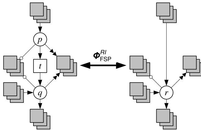
Fig. 24. One of the liveness and boundedness preserving reduction rules presented in [75]: Fusion of Series of Places (FSP).
