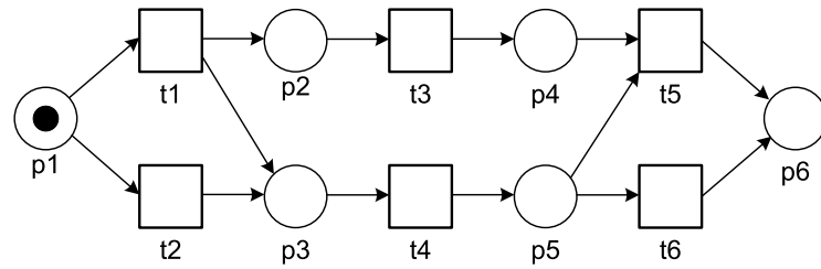
(a) a relaxed sound WF-net
