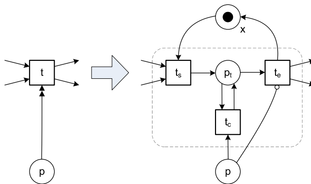
Fig. 9. Construction showing that reset arcs can be translated into inhibitor arcs.
