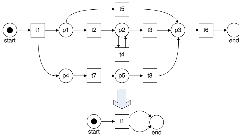
Fig. 22. A WF-net that is not sound and that cannot be reduced completely.
