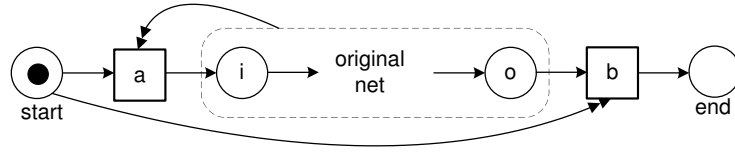
Fig. 15. Failed attempt to show that generalized soundness is undecidable for WF-nets with reset arcs.
