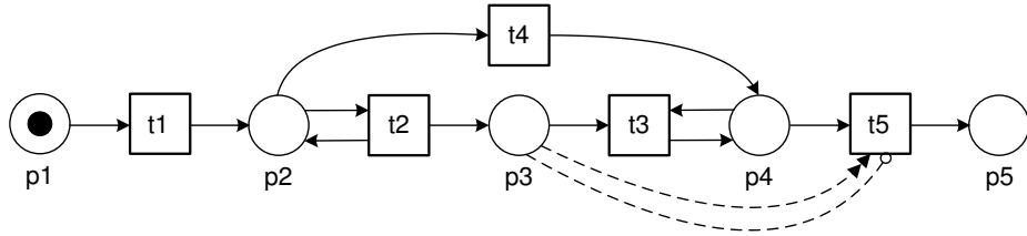
Fig. 19. N is the WF-net without the reset/inhibitor arc, N_R is the net with the reset arc, N_I is the net with the inhibitor arc, and N_{RI} is the net with both the reset arc and inhibitor arc.
