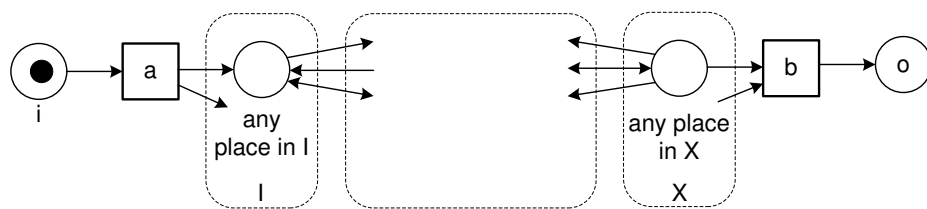
Fig. 18. Construction showing that easy soundness is undecidable for WF-nets with reset arcs.
