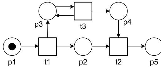
(b) a lazy sound net
