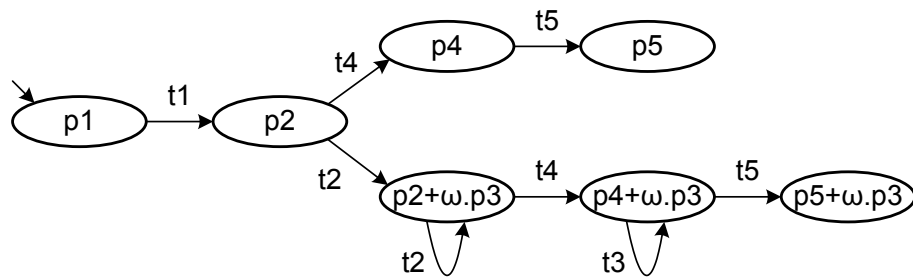
Fig. 20. The coverability graph of N .
