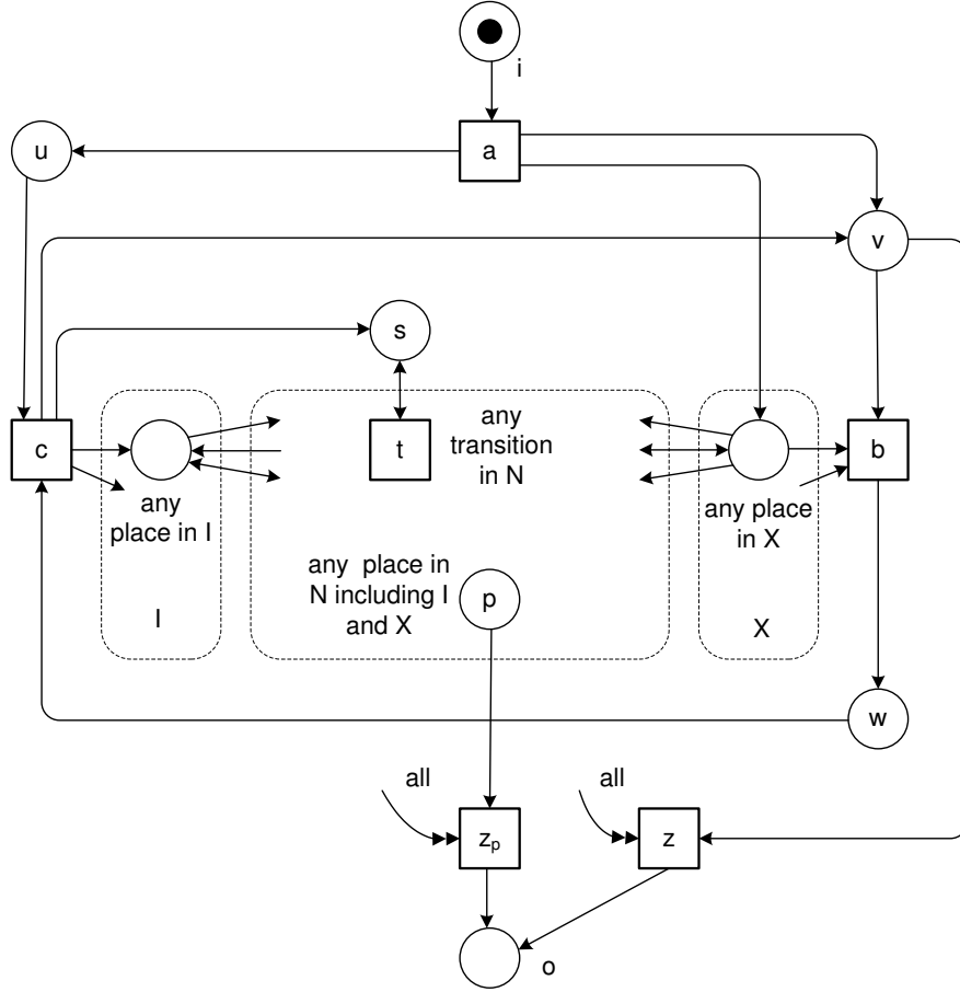
Fig. 10. Construction showing that soundness is undecidable for WF-nets with reset arcs. The original net comprises the three dashed areas: I is the set of places of N initially marked, X is the set of places that are marked in M_X , and all other nodes of N are shown in the dashed area in the middle. Note that I and X may overlap.
