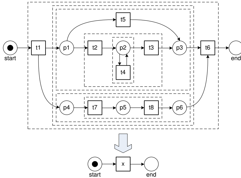
Fig. 21. A sound WF-net that can be reduced to the trivially correct WF-net.
