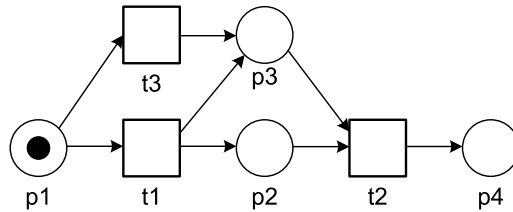
(c) an easy sound net
