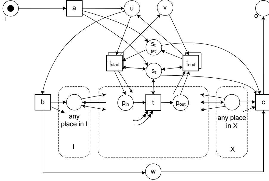
Fig. 16. Construction showing that reachability can be expressed in terms of relaxed soundness for WF-nets with reset arcs.
