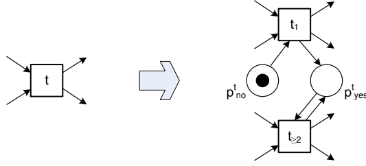
Fig. 17. Construction showing that relaxed soundness is decidable for WF-nets without reset/inhibitor arcs, i.e., t is involved in a “good run” in the original model (left) if and only if [o, p_{yes}^t] is reachable in the adapted model (right).
