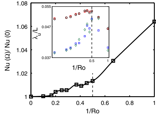
FIG. 1 (color online). The ratio Nu(\Omega)/Nu(\Omega = 0) as a function of 1/Ro for Ra = 4 \times 10^7 and Pr = 6.26 . Open black squares indicate the numerical results. The numerical error is approximately 0.2%, which is indicated by the size of the symbols. Inset: The thickness of the kinematic top and bottom BLs based on the maximum rms azimuthal [upper symbols: black circles (red squares) for top (bottom) BL] and radial [lower symbols: green diamonds (blue squares) for top (bottom) BL] velocities. The vertical dashed lines in both graphs represent 1/Ro_c and indicate the transition in boundary-layer character from Prandtl-Blasius (left) to Ekman (right) behavior.
