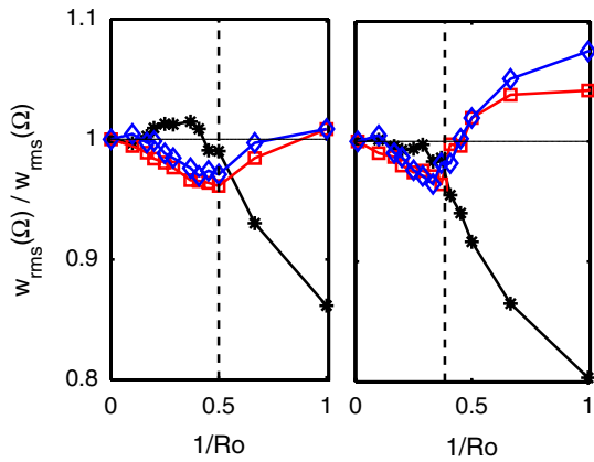
FIG. 3 (color online). The normalized averaged rms vertical velocities w_{\text{rms}} for \text{Ra} = 4 \times 10^7 (left) and \text{Ra} = 2.73 \times 10^8 (right) as a function of 1/\text{Ro} . The black line (with asterisks) indicates the normalized volume-averaged value of w_{\text{rms}} . The red line (with squares) and blue line (with diamonds) indicate the normalized horizontally averaged w_{\text{rms}} at the edge of the thermal BL based on the slope at, respectively, the lower and upper plate. The vertical dashed lines again indicate the position of 1/\text{Ro}_c .
