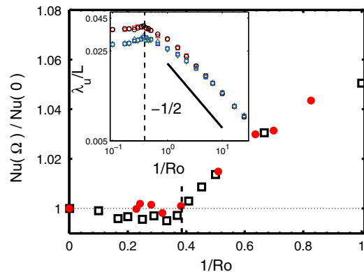
FIG. 2 (color online). Nu(\Omega)/Nu(\Omega = 0) for Ra = 2.73 \times 10^8 and Pr = 6.26 . Red solid circles: experimental data ( T_m = 24^\circ\text{C} and \Delta = 1.00\text{ K} ). Open black squares: numerical results. The experimental error coincides approximately with the symbol size, and the numerical error is approximately 0.5%. Inset: Thickness of the kinetic BL. For dashed vertical lines and inset, see Fig. 1.
