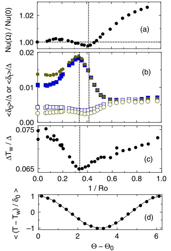
FIG. 4 (color online). Results for \text{Ra} = 9.0 \times 10^9 and \text{Pr} = 4.38 ( T_m = 40.00^\circ\text{C} , \Delta = 16.00\text{ K} ). (a) \text{Nu}(\Omega)/\text{Nu}(\Omega = 0) vs 1/\text{Ro} . The error bar is smaller than the size of the symbols. (b) Solid symbols: time-averaged LSC amplitudes \langle \delta_0 \rangle / \Delta ( z = 0 , circles) and \langle \delta_i \rangle / \Delta ( z = L/4 , squares) as a function of 1/\text{Ro} . Open symbols: rms fluctuations about the cosine fit [Eq. (1)] to the temperature data. (c) Vertical temperature variation \Delta T_w / \Delta along the sidewall. (d) Circles: time-averaged normalized sidewall-temperature profile \langle [T(\theta) - T_w] / \delta_0 \rangle at the horizontal midplane for 1/\text{Ro} = 1 determined as in [15]. Solid line: \cos(\theta - \theta_0) .
