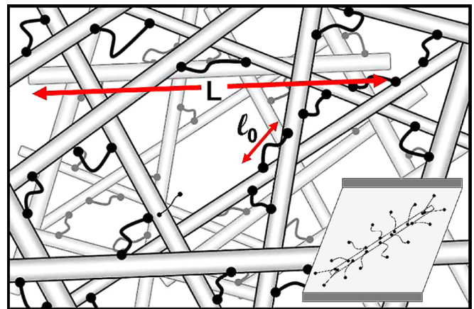
FIG. 1 (color online). Schematic figure of an isotropic stiff polymer network with highly compliant cross-linkers. The inset illustrates the proposed nonuniform deformation of the cross-linkers on a single filament in a sheared background medium.
