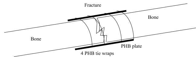
fig. 1 New design for fixation of fractured bones
