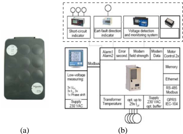
Figure 4. Black box solutions for distribution automation
