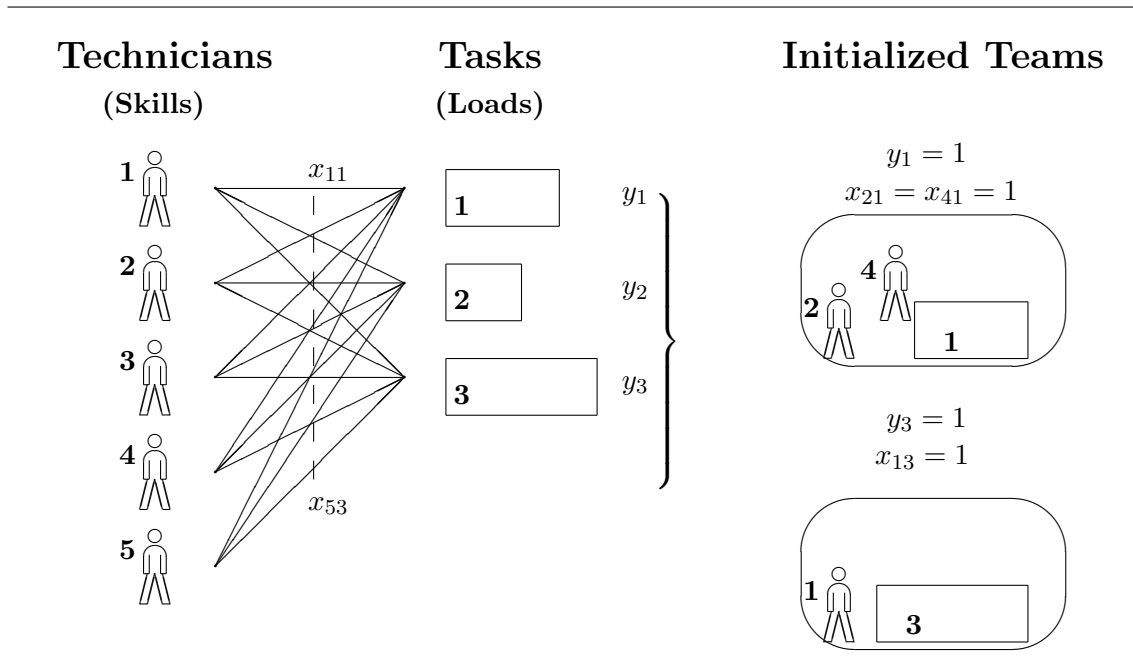
Figure 2: Initializations of teams in the IMM
