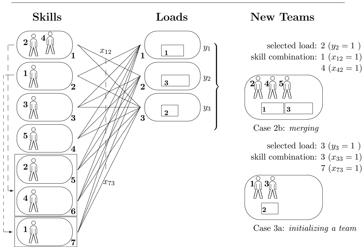
Figure 3: Extending partial schedule with the FMM (Scenario 1)
