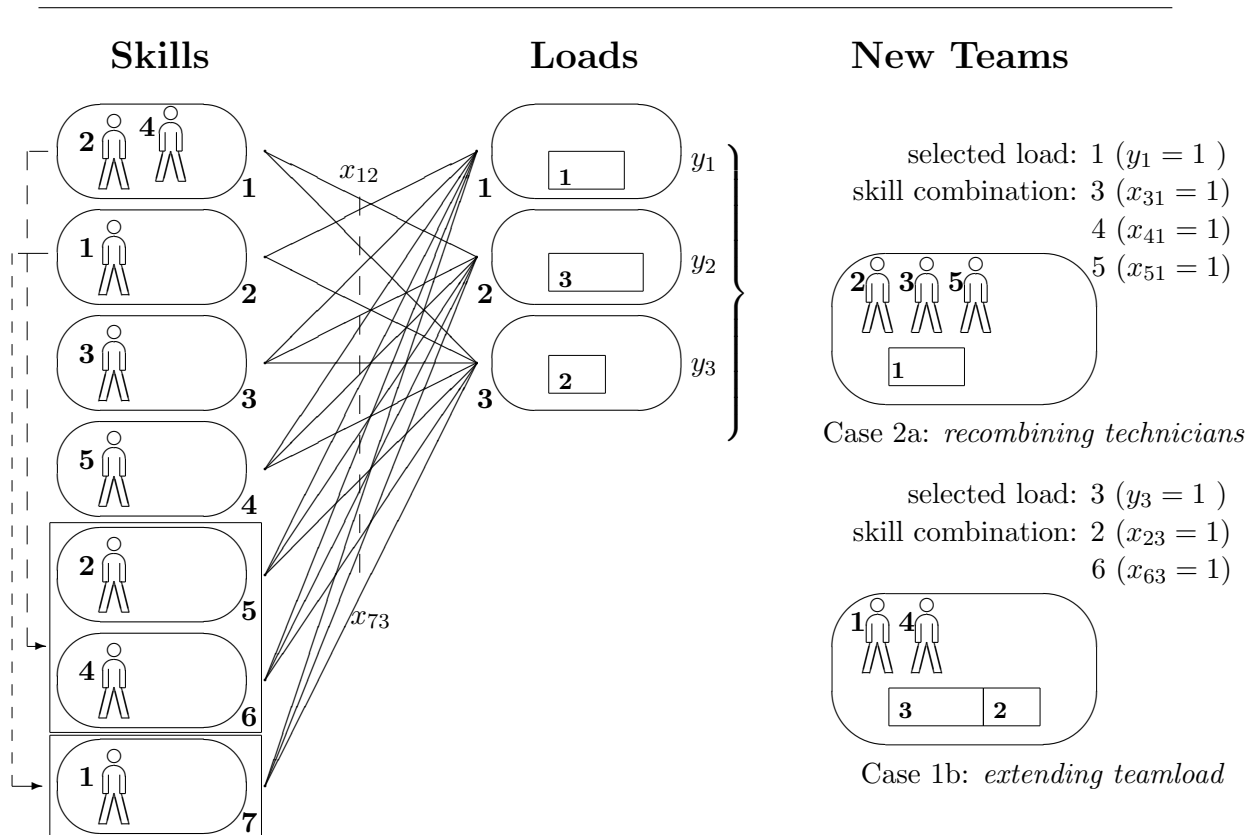
Figure 4: Extending partial schedule with the FMM (Scenario 2)
