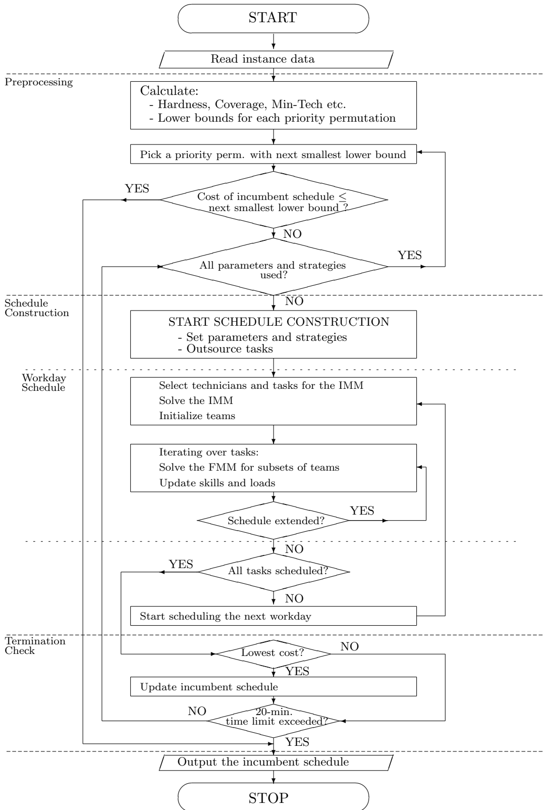
Figure 1: Flowchart of the Combinatorial Algorithm
