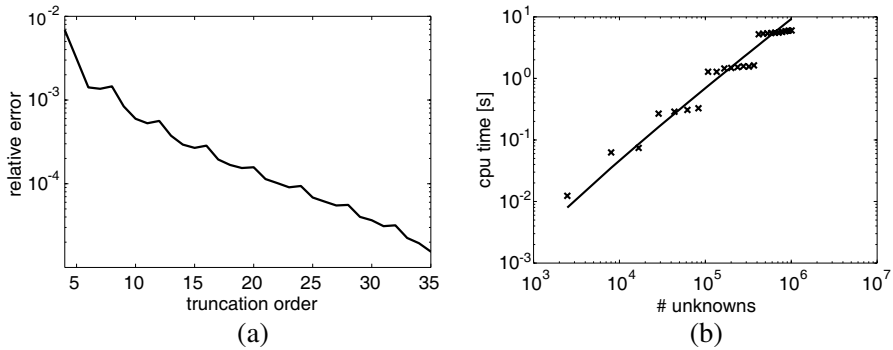
Figure 4. (a) Relative error versus the truncation order in the Fourier modes for an array of cavities with circular cross section. (b) CPU time per matrix-vector product versus total number of unknowns. The solid line is given by \alpha N \cdot M \log(M) , with M the total number of modes and N the number of samples in z . The solid line corresponds to the asymptotic complexity estimate of the matrix-vector product.
