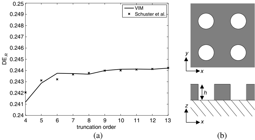
Figure 3. (a) Zeroth-order diffraction efficiency in reflection versus the truncation order in the Fourier modes for an array of cavities with (b) circular cross section, compared to the results by Schuster et al. [5].
