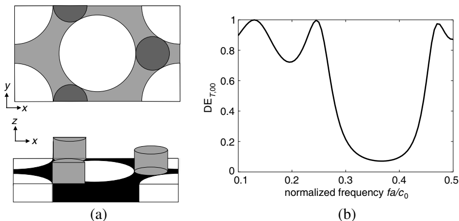
Figure 5. (a) Top and side view of a layer of pillars on top of a layer with holes in an face-centered cubical lattice. (b) Zeroth order diffraction coefficient in transmission for a configuration consisting of three layers of the structure on the left, each one shifted over one-third of a period in the x -direction.
