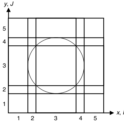
Figure 1. Circular geometry captured on a tensor grid.
