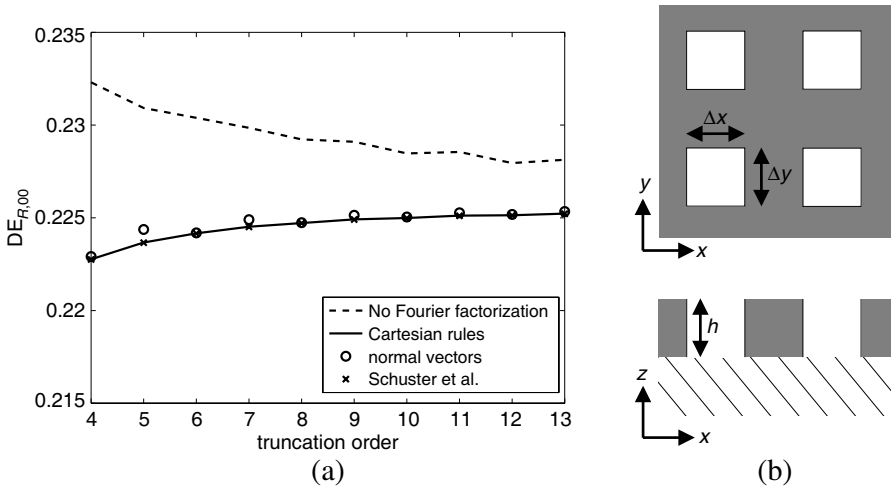
Figure 2. (a) Zeroth-order diffraction efficiency in reflection versus the truncation order in the Fourier modes for an array of cavities with (b) square cross section, compared to the results by Schuster et al. [5].
