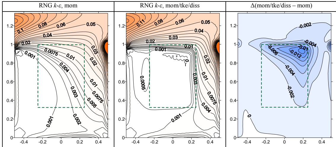
Figure 5. Normalized dissipation rates \varepsilon H/U_H^3 for the RNG k-\varepsilon turbulence model simulations.
