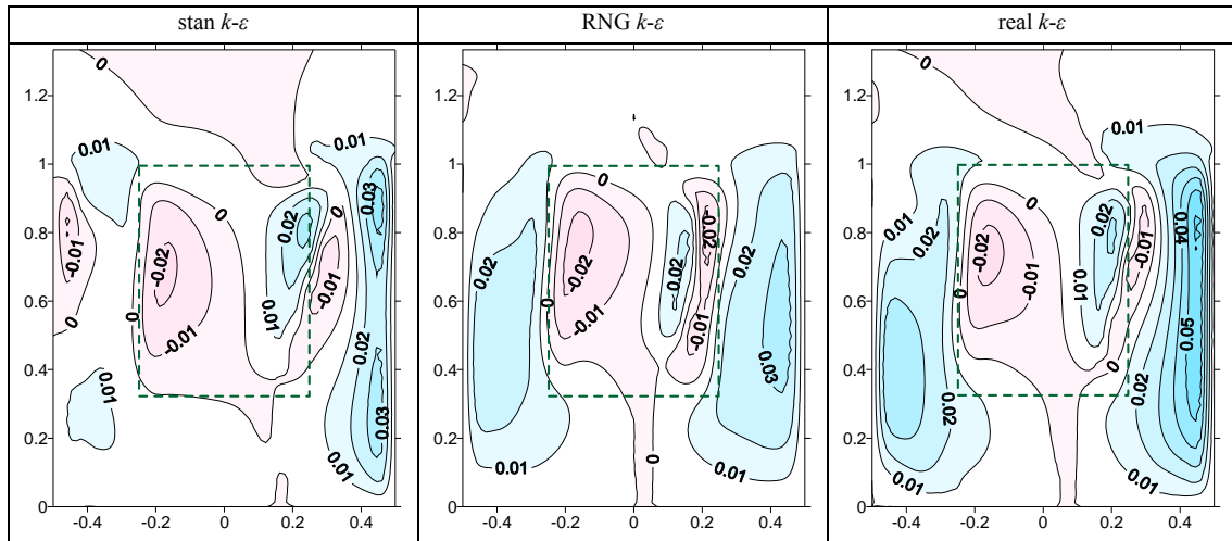
Figure 3. Normalized differences \Delta U_3/U_H (Equation 4) between simulations with the full set of vegetation terms (Equation 1-3) and the extra terms in the momentum equations only (Equation 1).
