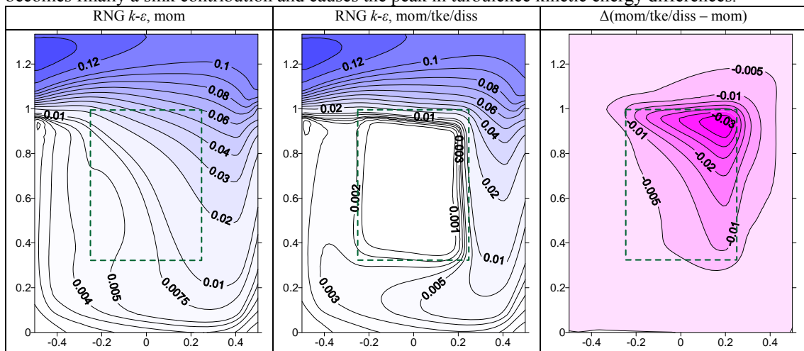
Figure 4. Normalized turbulence kinetic energy k/U_H^2 for the RNG k-\epsilon turbulence model simulations.
