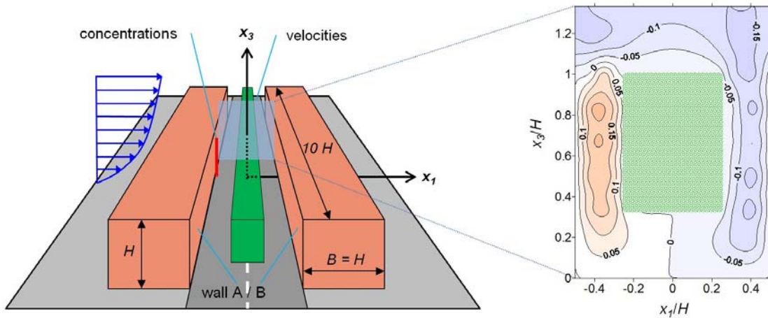
Figure 1. Isolated street canyon model with avenue-trees (left), and normalized vertical velocities U_3/U_H from wind tunnel measurements (right).
