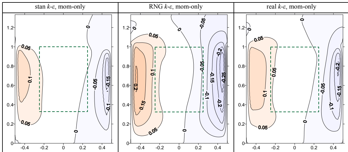
Figure 2. Simulated normalized vertical velocities U_3/U_H in the vertical plane at x_2/H = 0.5 (Figure 1) with the extra terms in the momentum equations only (Equation 1).
