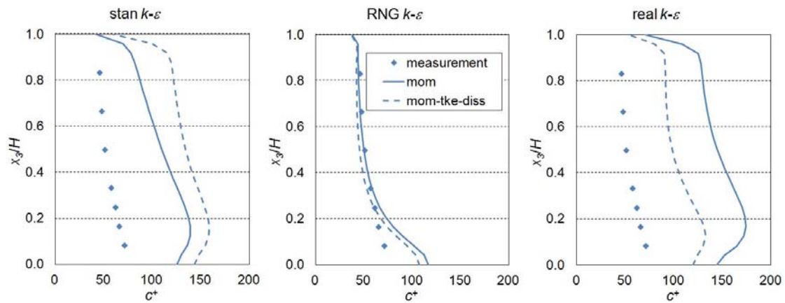
Figure 6. Normalized pollutant concentrations c^+ close to the wall A (Figure 1).
