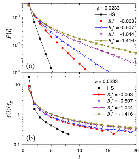
FIG. 3 (color online). (a) The probability of finding a transient cluster of size i and (b) the average cluster lifetime (normalized by the Brownian time \tau_B = a^2/D_c ) as a function of i for hard spheres and for four different interparticle attractions. The particle volume fraction is \phi = 0.0233 .
