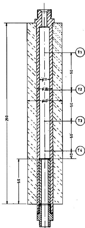
Fig. 2.2 Tubular fixed bed reactor.
