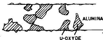
Fig. 3.13 Uranium oxide crystallites in alumina matrix.
