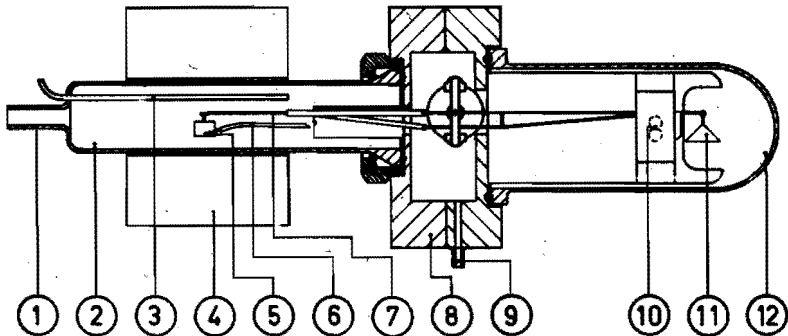
Fig. 2.6 Thermobalance:
