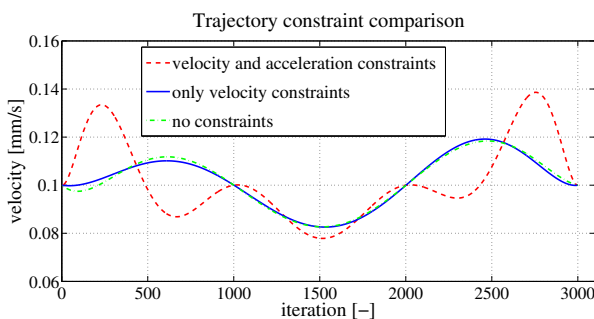
Figure 5. Polynomial constraint comparison. The dashed (red) line shows that with acceleration and velocity constraints on feature points, an overall oscillating velocity signal is computed. The solid (blue) line shows that only constraints on velocity give the most moderate velocity trajectory.
