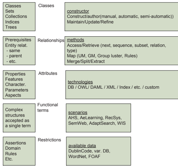
Fig. 4. Domain Model abstraction class
