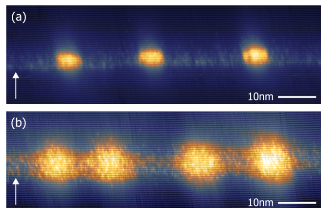
FIG. 1. Topographic XSTM images of two typical stretches of the QD layer in (a) the as grown and (b) the annealed sample. The arrows indicate the growth direction.
