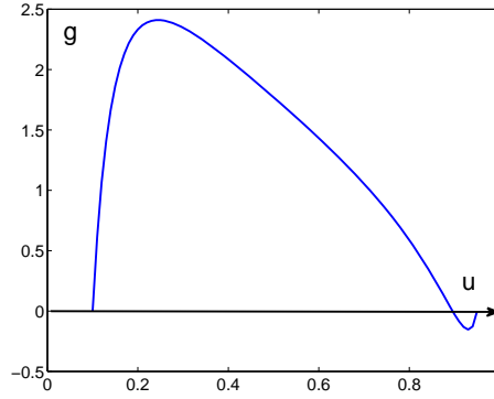
FIGURE 2.2: THE FUNCTION g(u) FOR p = 0.5 , q = 0.5 , M = 2 , u_r = 0.1 , u_\ell = 0.95 AND HENCE, BY THE RH-CONDITION (2.1.4), s = 1.12
