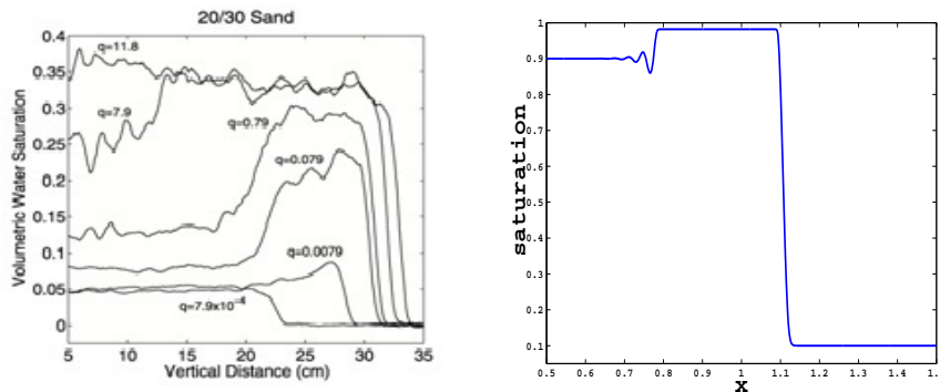
FIGURE 1.1: SATURATION OVERTHOOT PROFILES: EXPERIMENTAL RESULTS IN [5] (LEFT), A NUMERICAL EXAMPLE (RIGHT)
