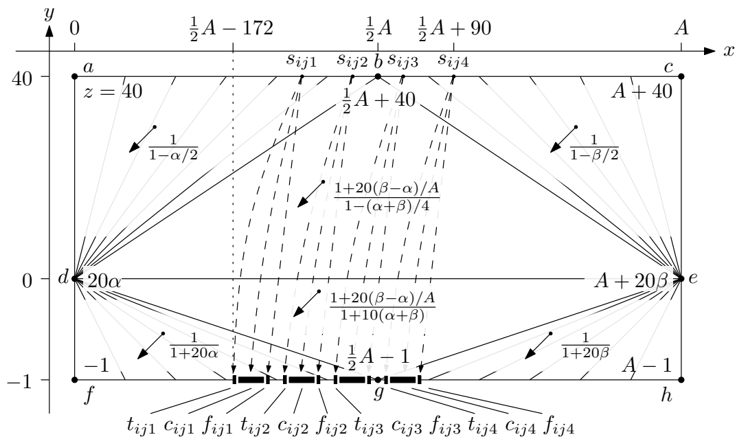
Figure 6: Distances and gradients on a connector gadget. All coordinates are relative to the lowermost position of the control vertex d = v_{i(j-1)} . The other control vertex is e = v_{ij} . Thus, e and d are the only imprecise vertices. The x - and y -coordinates of the vertices are indicated on the axes. The elevations of the key vertices are written next to the vertices. The elevations of the control vertices are expressed as a function of \alpha, \beta \in [0, 1] . The directions of steepest descent on the different faces of the gadget (marked with arrows) are expressed in the form dx/dy , as a function of \alpha and \beta .
