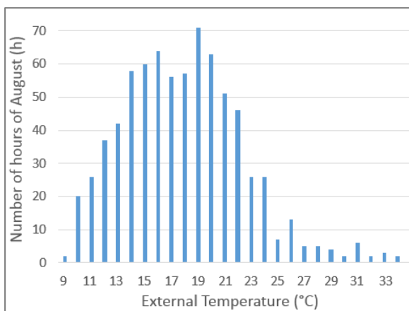
Figure 4: Histogram of external air temperatures during the month of August
