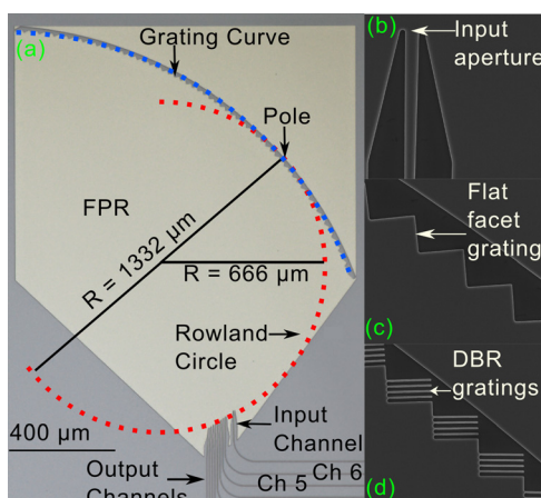
FIG. 1. (a) A microscopic image of the fabricated PCG illustrating the various parts, (b) an image of the input aperture, (c) an image of the fabricated flat facet grating, and (d) an image of the fabricated DBR facet grating.
