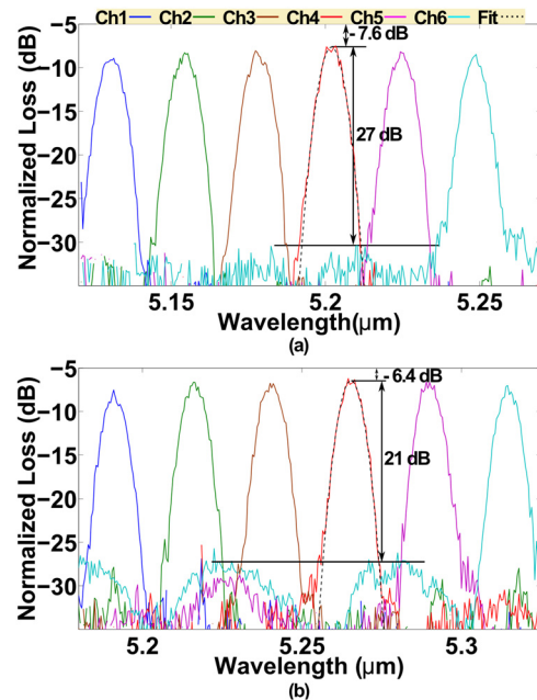
FIG. 2. Normalized spectra of a six channel PCG with flat grating facets for (a) TE polarized light and (b) TM polarized light.
