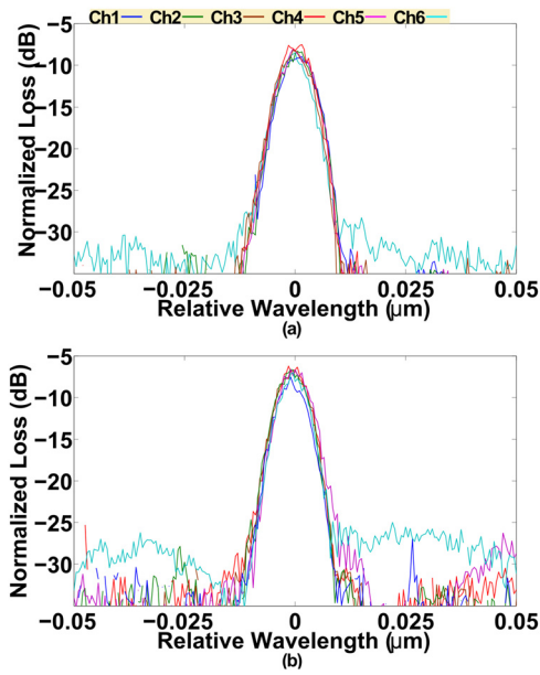
FIG. 3. Overlapped spectra of the six channel PCG with flat grating facets for (a) TE polarization and (b) TM polarization.
