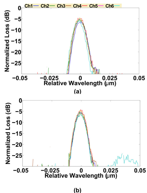
FIG. 6. Overlapped spectra of the six channel PCG with DBR gratings for (a) TE polarization and (b) TM polarization.
