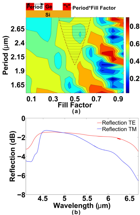
FIG. 4. (a) Simulated contour plot of reflectivity from a four period DBR grating as a function of period and fill factor. The shaded area shows the combination which can be fabricated using 1-line contact lithography and the schematic at top explains grating parameters. (b) Simulated broadband reflection spectrum of a four period DBR grating with a period of 2.15 \mu\text{m} and 50% fill factor for TE and TM polarized light.
