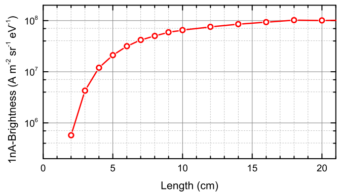
FIG. 8. (Color online) Brightness for different MOC lengths. The other parameters can be found in Table II except for r = 1.0 mm, \theta = 36 mrad and \nabla B = 2.0 T/m. Increasing the MOC length does improve the brightness but not to a great extent.
