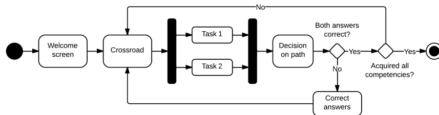
Fig. 2. Game sequence
