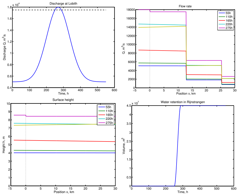
Figure 17: Flooding scenario reaching 18000 \text{m}^3/\text{s} in 11.5 days at proposed design peak discharge of 17500 \text{m}^3/\text{s} . Top left: discharge scenario at Lobith. Top right: flowrates throughout the domain at sequential times; discontinuities occur at channel bifurcation points. Bottom left: free surface height in the domain at sequential times; discontinuity at x = 0 due to removal to Rijnstrangen retention area. Bottom right: volume of water retained in Rijnstrangen area as a function of time.
