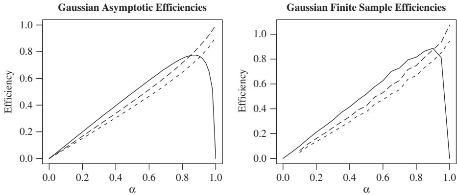
Fig. 2. Asymptotic (left panel) and finite sample (window width 20, right panel) efficiencies for Q_{adj}^\alpha (solid), TM_{adj}^\alpha (short dash) and TMS_{adj}^\alpha (long dash), for varying \alpha .
