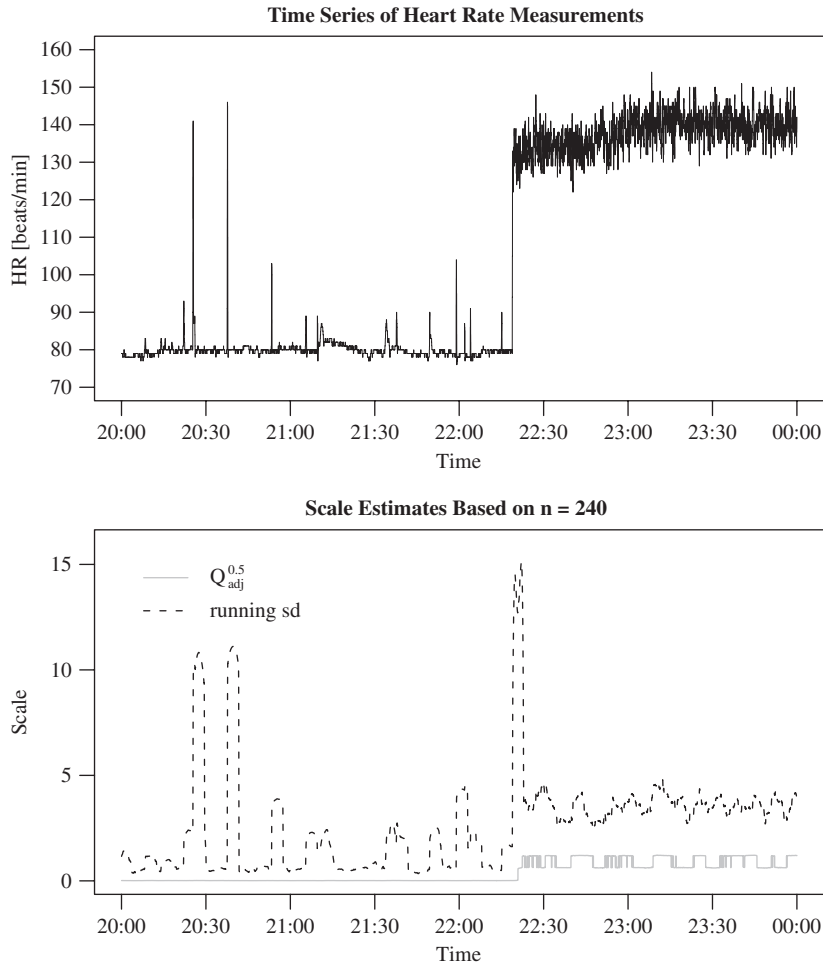
Fig. 8. Physiological data (top panel). The bottom panel presents the scale as estimated by the Q_{adj}^{0.5} estimator and the residual standard deviation after an OLS-fit with n = 240 .
