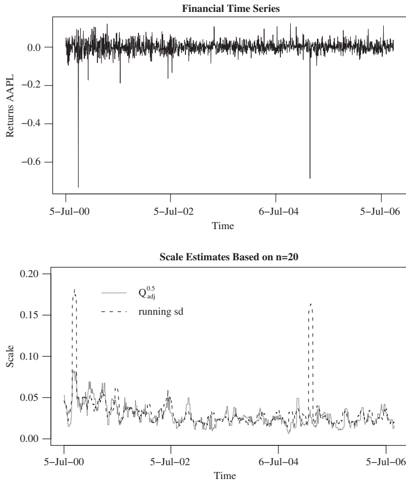
Fig. 7. AAPL stock returns (top panel). The bottom panel presents the scale as estimated by the Q_{adj}^{0.5} estimator and the residual standard deviation after an OLS-fit with n = 20 .
