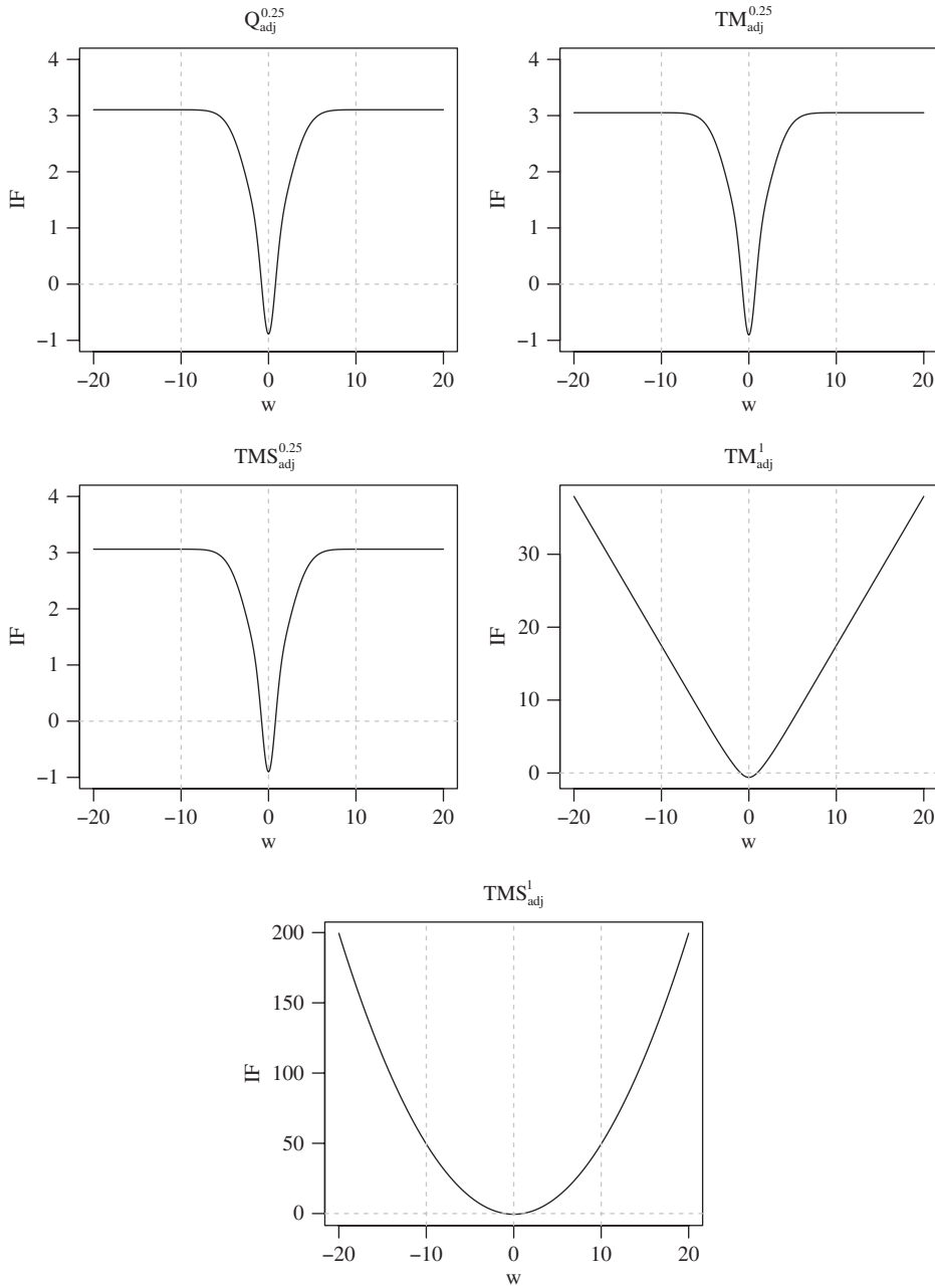
Fig. 1. Influence functions for the Q_{adj}^z , TM_{adj}^z , and TMS_{adj}^z estimator, for \alpha = 0.25 and for \alpha = 1 .
