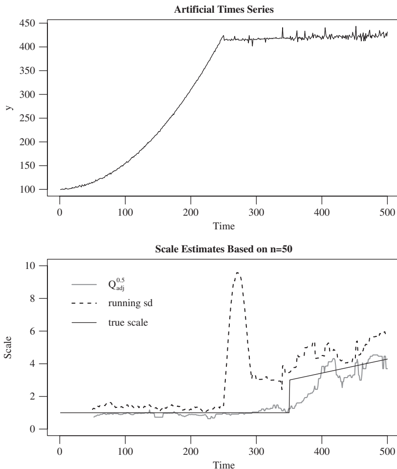
Fig. 6. Artificial time series (top panel). The bottom panel presents the scale as estimated by the Q_{adj}^{0.5} estimator and the residual standard deviation after an OLS-fit with n = 50 . The true scale is represented by the thin solid line.
