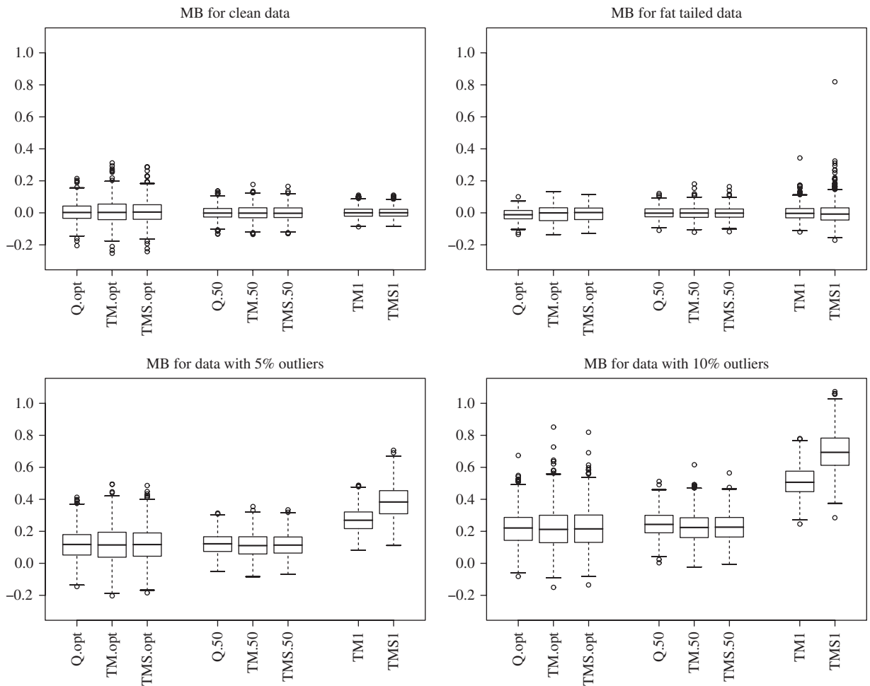
Fig. 3. Boxplots of 1000 values of the mean bias (MB) for simulation schemes using clean data (top left), fat tailed data (top right), data with 5% outliers (bottom left) and 10% outliers (bottom right). In every graph, the first three boxplots present the MB for the Q_{adj}^z , TM_{adj}^z and TMS_{adj}^z estimators with optimal fsbp; the middle three for \alpha = 0.5 ; the last two for the non-robust TMI_{adj}^1 and TMSI_{adj}^1 .
