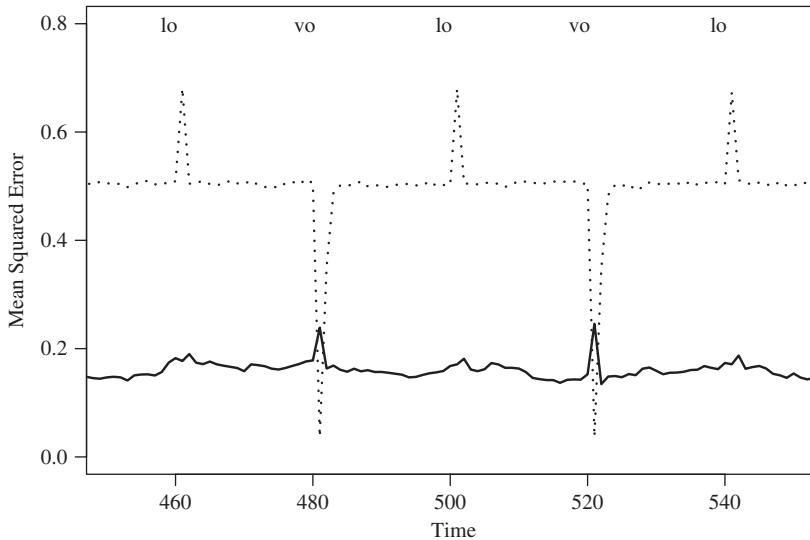
Fig. 5. Average value of MSE_t evaluated from N_s = 1000 simulation runs for the time period 440–560 for the Q_{adj}^{0.5} estimator (solid line) and the ML estimator of a GARCH(0, 1) model (dotted line), in the presence of level outliers (lo) and volatility outliers (vo).
