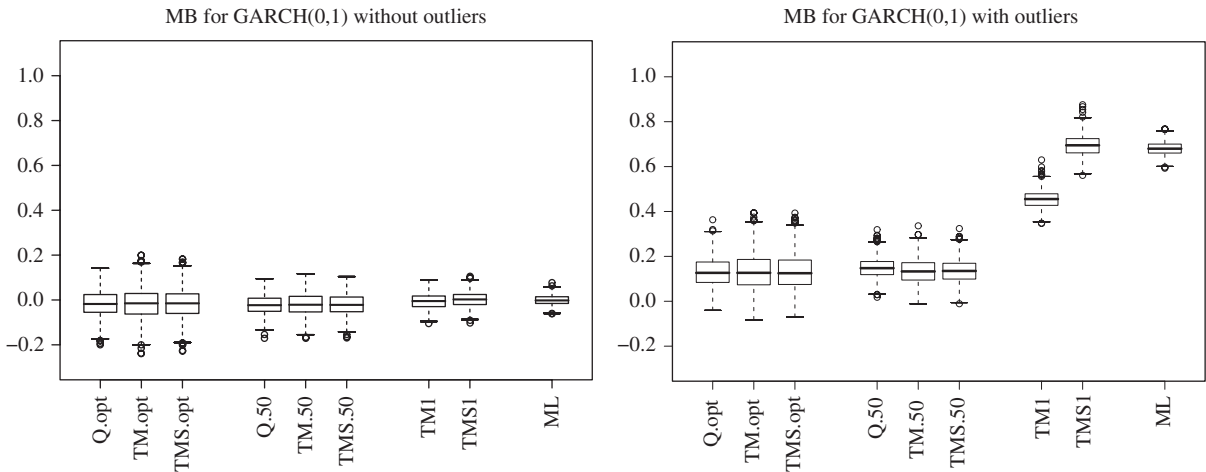
Fig. 4. As Fig. 3, but now for clean data (left) and 5% contaminated data (right) from a GARCH(0, 1) model, and with the last boxplot corresponding to the ML estimator.
