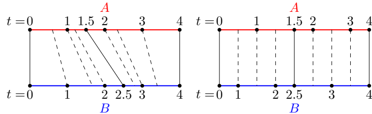
■ Figure 3 A piecewise linear matching of timestamps. Left, the matching drawn with the original time axes. Right, the matching drawn after warping the time axes.
