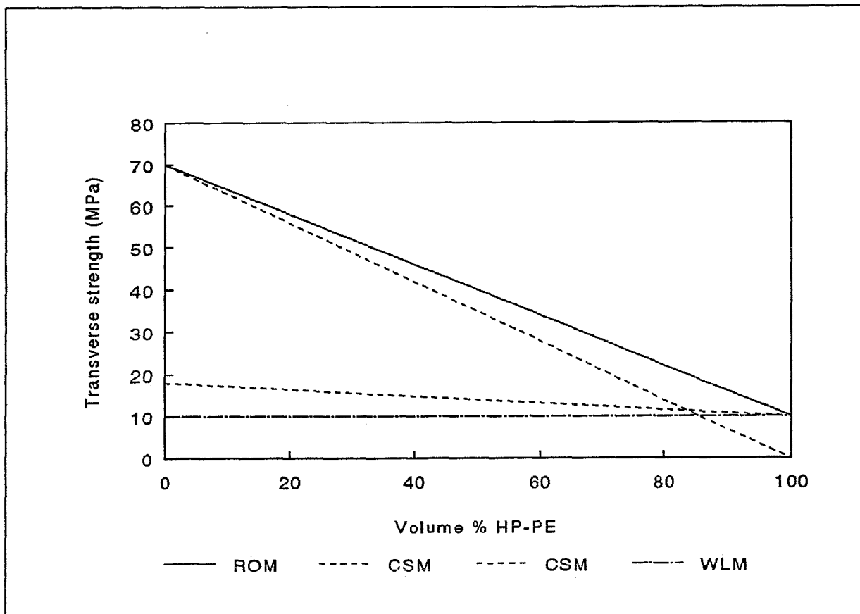
Fig. 2 Transverse strength vs. hybrid composition
