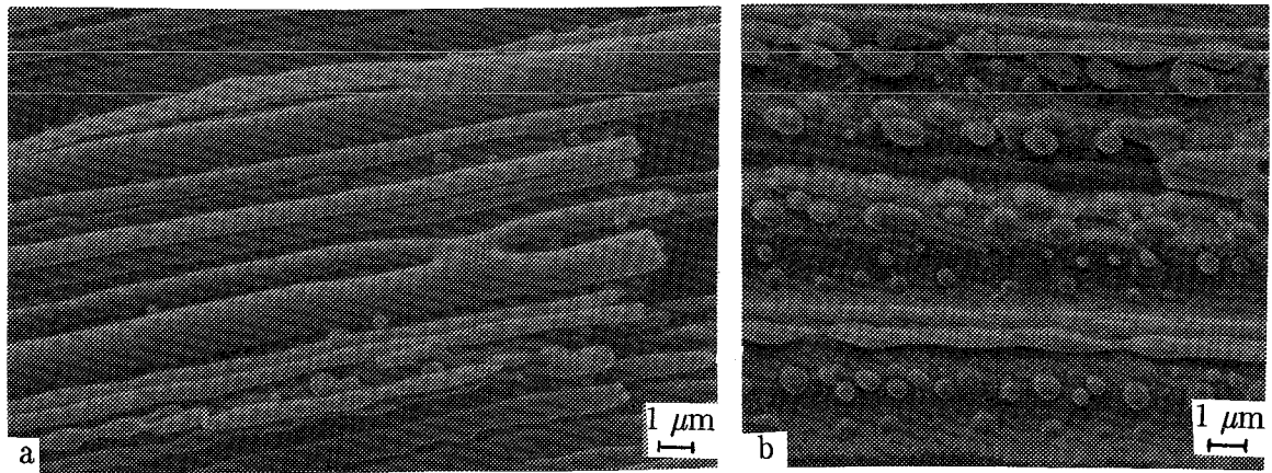
Figure 4.41 Breaking PS threads in a HDPE matrix. The blends were prepared using a corotating twin screw extruder with: a) quenching immediately after the die or b) several seconds between die and waterbath (Meijer et al. 1988). Reprinted with permission of Hüthig und Wepf Verlag.
