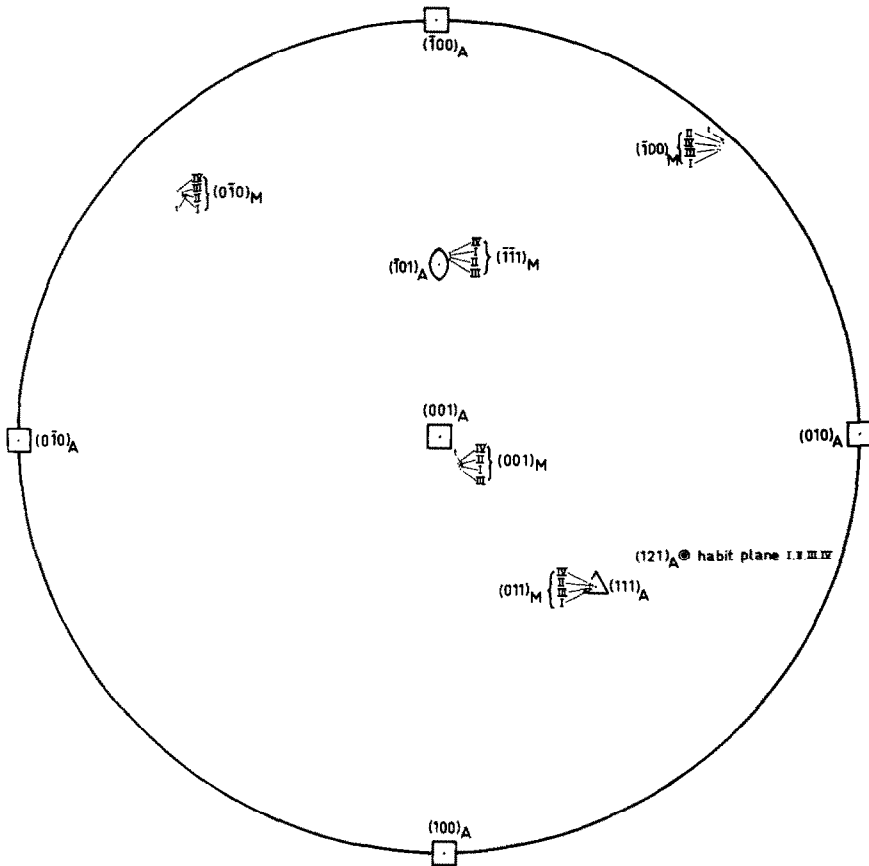
Fig. 9. Orientation relations of the martensite needles of the specimen of Fig. 4. The martensite orientation predicted by the I.P.S. theory for \delta = 1 is indicated with l .
