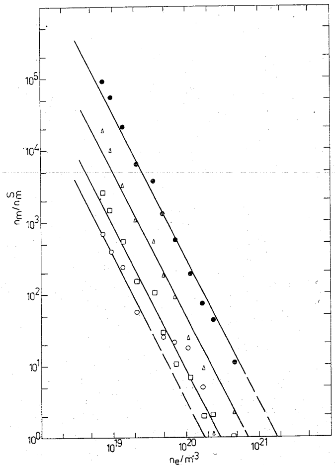
Fig. 1. The ratios n_m/n_m^S , excited group density normalized to its Saha-density, as functions of the electron density n_e for the 4p (●), 4d (△), 5d (□) and 6d (○) group. The solid lines are according to an n_e^{-2} slope. T_e = 3.5 \text{ eV} and n_a = 10^{19} \text{ m}^{-3} .
