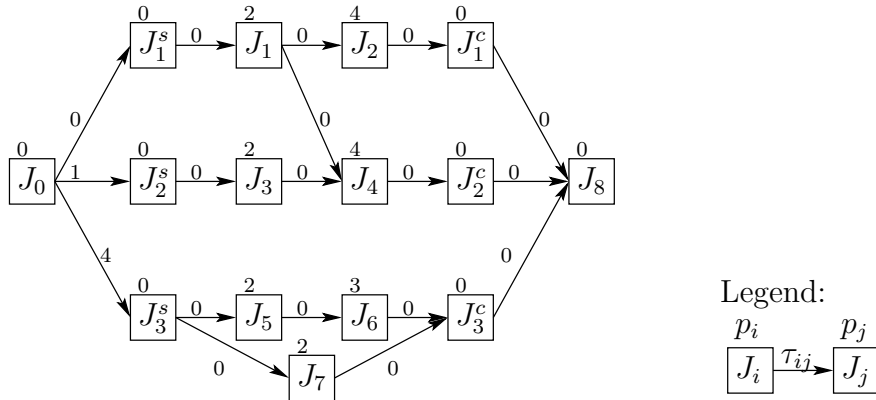
Figure 1: Example project: Activity-on-Node representation.
