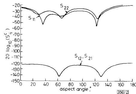
Fig. 2 Variation of 20 \log_{10} |S_{ij}^c| with aspect angle for achiral sphere of radius \lambda \mu_r = 1 ; \epsilon_r = 4 ; \alpha = \beta
