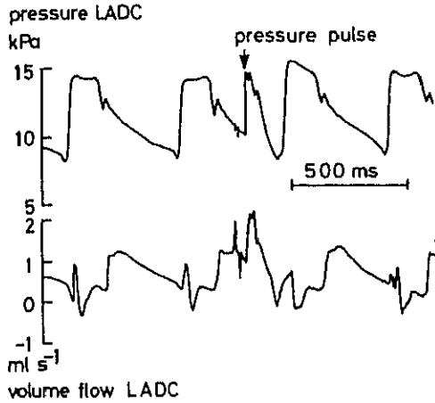
FIG. 2. Pressure ( P_1 ) and volume flow curves proximal in the LADC. The recorded pressure pulse arrived approximately 100 ms after closure of the aortic valve. The rising slope of this pressure pulse is shown in more detail in Fig. 3A.
