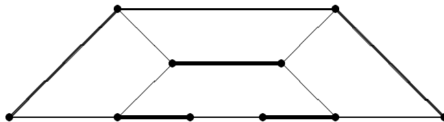
Figure 2: A maximum matching.
