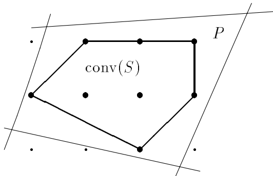
Figure 1: P , S , and \text{conv}(S) .
