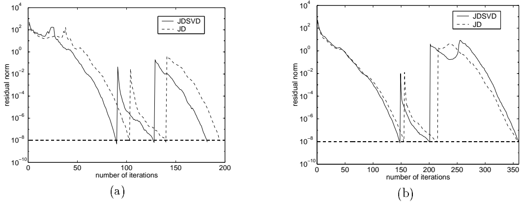
FIG. 8.2: (a) JDSVD (solid) and JD (dashed) for the three largest \sigma 's of \text{diag}(1..1000) . (b) The same as Figure 8.2(a), only with \text{GMRES}_2 to solve the correction equation.
