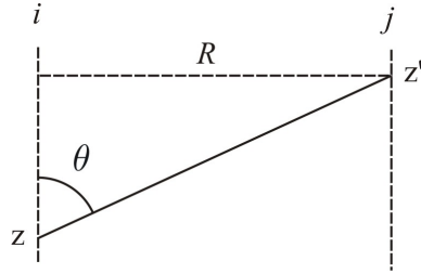
Figure 4.9.: Overview of integration variables in calculation of U_{ij} .
