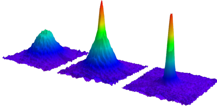
Figure 1.1.: Absorption image of trapped atoms around the critical temperature. In the horizontal plane are two spatial dimensions, with the total absorption along the third dimension on the vertical axis. After switching off the trap the gas cloud can expand enough to take an absorption image. The leftmost picture shows an uncondensed cloud, with a temperature just above the transition point, which is at about 2\mu\text{K} . The middle picture shows a cloud just below the transition point and a condensate appears as a sharp peak in the middle, surrounded by a thermal cloud of uncondensed atoms. The rightmost picture shows a cloud cooled far below the transition temperature and nearly all atoms have condensed into the ground state, leaving a sharp peak. All pictures are about 1 mm across. Picture taken from [33].
