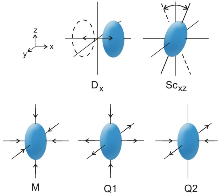
Figure 2.1.: Schematic illustration of the basic collective modes under consideration: the dipole mode D (shown here in the x -direction D_x ), scissors mode Sc (shown here in x - z plane Sc_{xz} ), the monopole mode M and the quadrupole modes Q_1 and Q_2 . These modes are discussed in more detail in Section 2.3.
