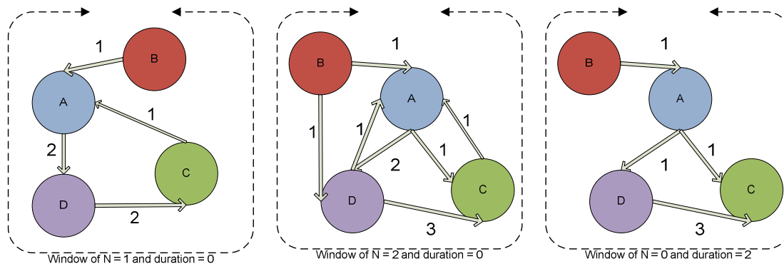
Figure 7: Different User Graph via different parameters
