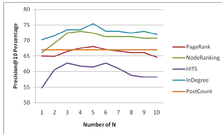
Figure 15: Comparison of algorithms with the variable N
