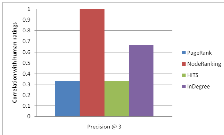
Figure 9: The performance of graph mining algorithms retrieving top 'Dell' buzz creators
