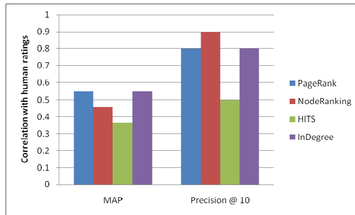
Figure 10: Comparison of results in topic 'Japan' for relevant comments
