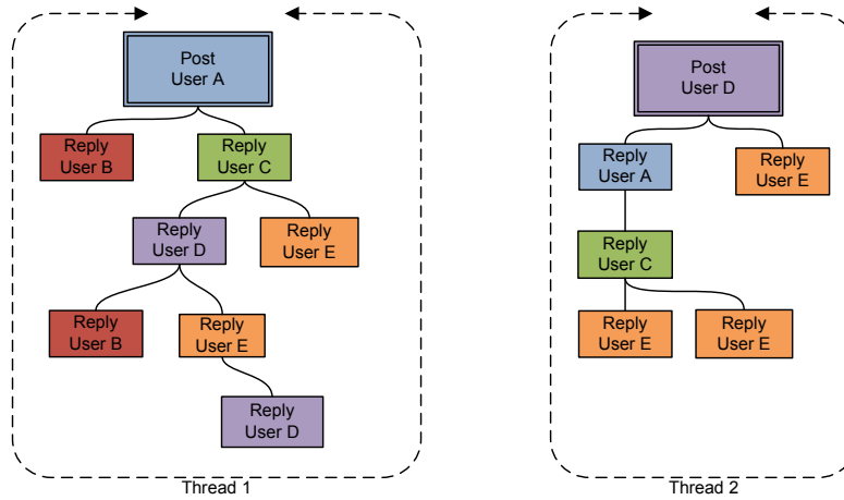
Figure 4: Graph construction example - 1.
