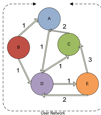
Figure 5: Graph construction example - 2.
