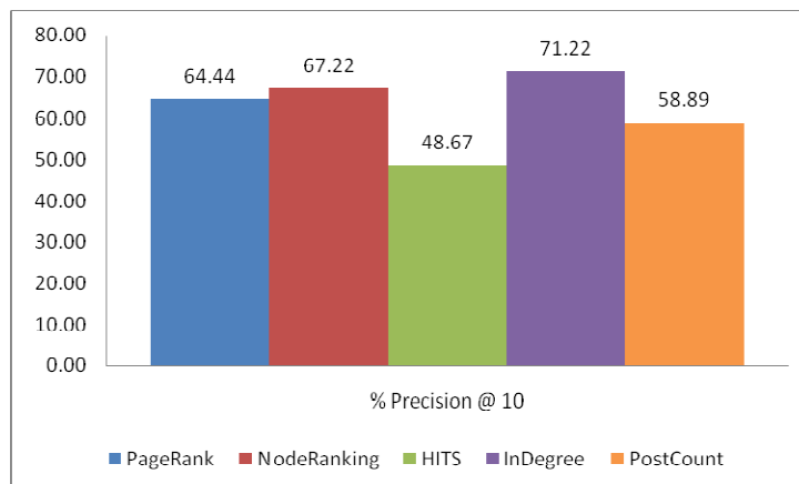
Figure 18: Algorithms' performance on topics which have less than 1500 posts
