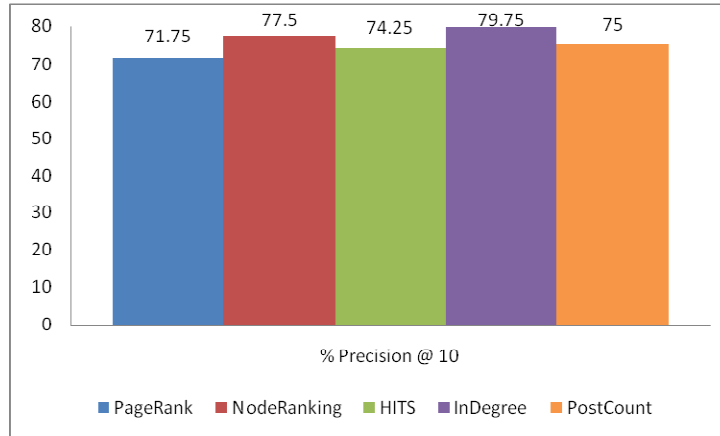
Figure 17: Algorithms' performance on topics which have greater than 1500 posts
