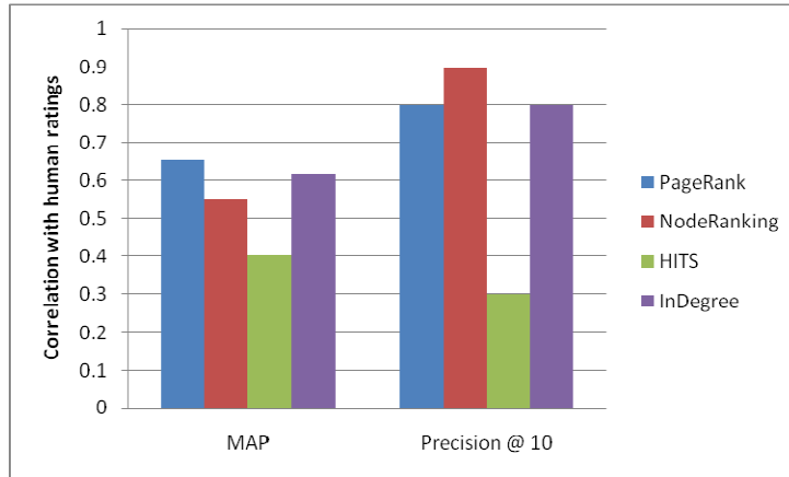
Figure 8: The performance of graph mining algorithms on 'Dell' topic
