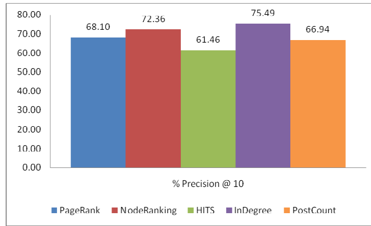
Figure 16: Comparison of algorithms' performances
