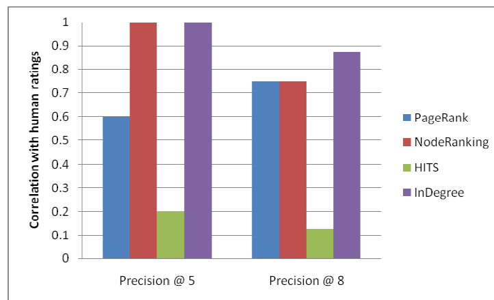
Figure 11: The performance of algorithms in retrieving top buzz creators for topic 'Japan'
