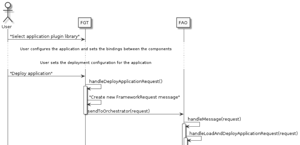
Figure 8: Sequence diagram of application deployment in the streaming framework
