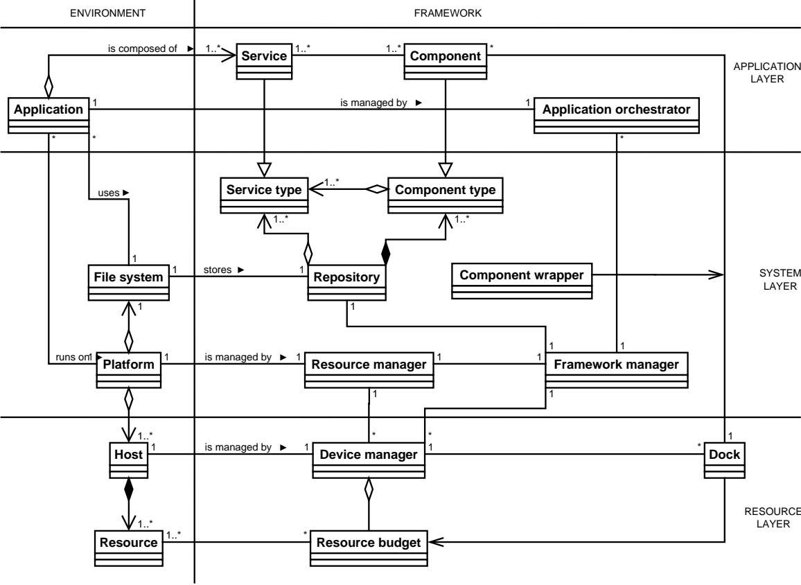
Figure 2: System overview
