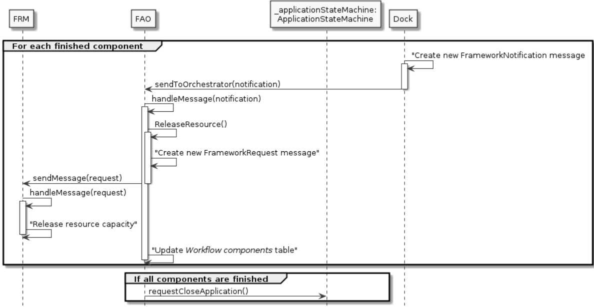
Figure 14: Sequence diagram of workflow finalization
