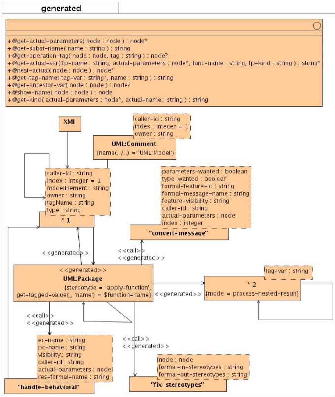
Figure 5.20: XSLT Template Flow of the Generated Script
