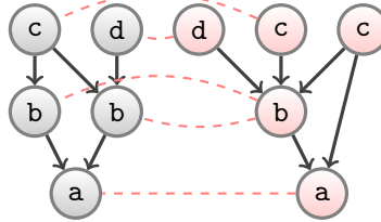
Figure 4.6: A graph is shown together with the maximum bisimulation graphs (highlighted) and a relation relating nodes from the graph with bisimilar equivalent nodes in the maximum bisimulation graph.
