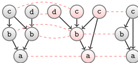
Figure 4.5: A graph consisting of two subgraphs is shown together with the maximum bisimulation graph (highlighted); also the relation relating index nodes with bisimilar equivalent graph nodes is shown.
