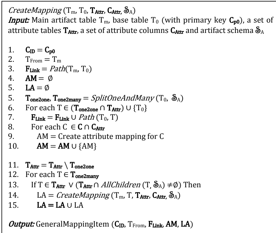
Figure 22: CreateMapping algorithm
