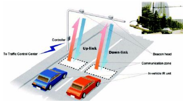
Figure 3-5 Infrared sensor
