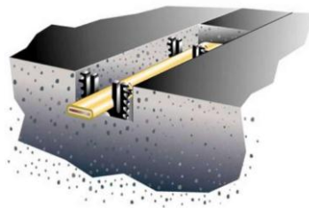
Figure 3-2 Piezoelectric sensor
