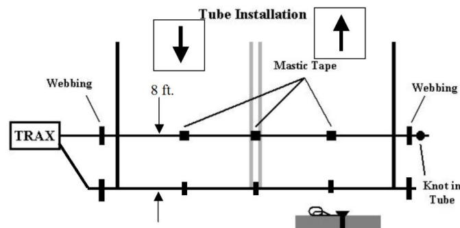
Figure 3-1 Road tube layout (Mcgowen & Sanderson, 2011)
