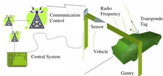
Figure 2 Complete RFID system connection [2].
