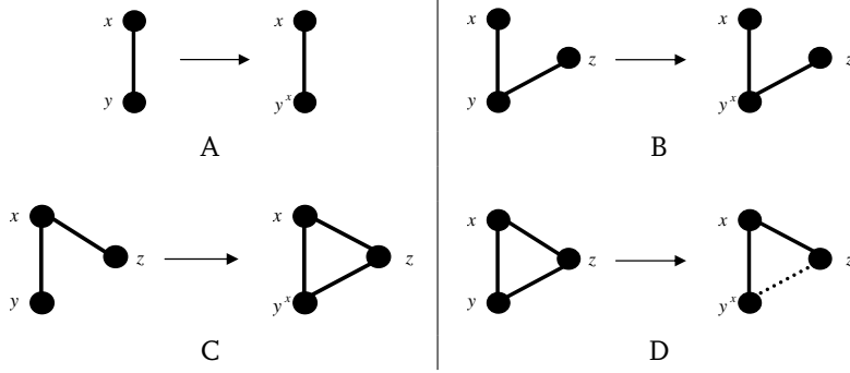
Figure 8.1: Replacing y by \exp(x, s)y
