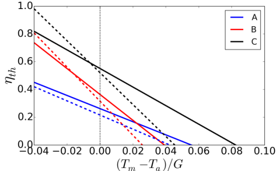
Figure 4: Collector curve for PVT collector A, B and C with a wind speed of 0 (solid) and 3 m/s (dashed), based on measured data from June 2015 to May 2016, with PV operational and measured in MPP
