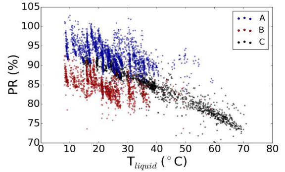
Figure 5: Correlation between the DC performance ratio and the average fluid temperature.
