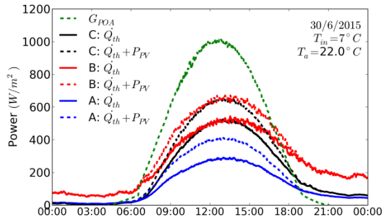
Figure 3b: Thermal (continuous lines, \dot{Q}_{th} ) and additional electrical power output (dashed lines, \dot{Q}_{th}+P_{PV} ) per m^2 for a day with a fluid input temperature of 7^\circ C . In-plane irradiance ( G_{POA} ) is shown in green.
