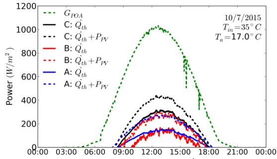
Figure 3a: Thermal (continuous lines, \dot{Q}_{th} ) and additional electrical power output (dashed lines, \dot{Q}_{th}+P_{PV} ) per m^2 for a day with a fluid input temperature of 35^\circ C . In-plane irradiance ( G_{POA} ) is shown in green.
