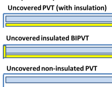
Figure 1: Three different PVT concepts (bright blue line: PV module, blue block: thermal absorber with fluid channels, yellow: insulation)
