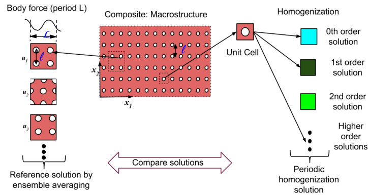
Figure 1: Schematic of the problem: Comparison of periodic homogenization solution with reference solution created by full-scale simulation for various scale ratios
