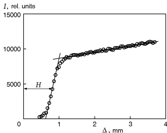
Fig. 5. Image density profiles illustrating the method of determining the distance H from the flame base to the rod end face.
