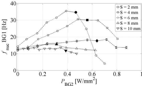
Figure 9. BG1 bubble frequency dependency on power fed to BG2 for varying inter-site distance S
