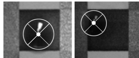
Figure 11. Natural nucleation site locations on BG1 observed during the experiments; Left) v_{bulk} = 0.45 m/s; Right) v_{bulk} = 0.85 m/s
