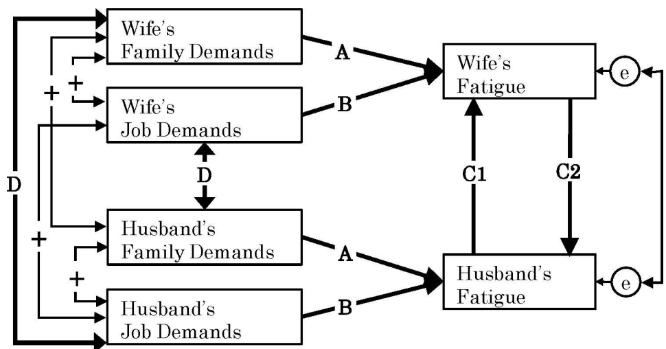
Fig 1. Hypothesis model.
