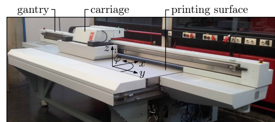
Figure 2: Océ Arizona 550 GT at the TU/e CST Motion Lab.
