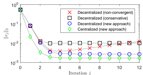
Figure 3: The importance of multivariable ILC design: i) ignoring interaction can lead to non-convergent schemes ( \times ); ii) appropriately accounting for interaction can improve performance ( \circ vs. \square ); and iii) centralized ILC ( \diamond ) yields the highest performance at the cost of increased modeling requirements.
