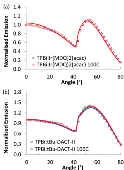
Fig. 6 Angular dependence of the p -polarised fluorescence of solution processed layers of host/guest systems with TPBi as host material, normalised at 0^\circ , for both not annealed layers (blue) and layers annealed at 100^\circ\text{C} (red). The dots represent the experimental measurements, the full lines the simulated results. There is no difference between annealed and non-annealed films.
