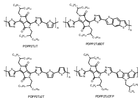
75 Fig. 1 Thiazole-bridged DPP-polymers as electron acceptor.
