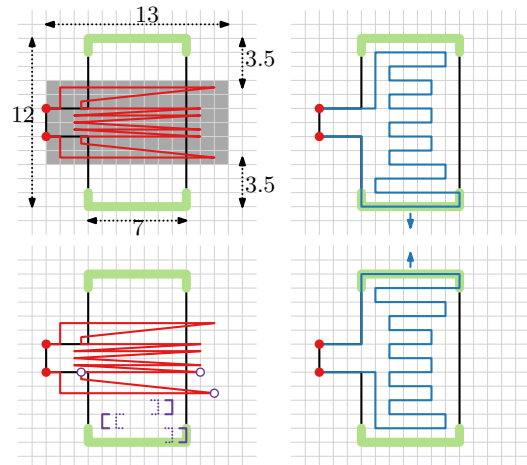
Figure 5: A propagation gadget. Specification and local curve (top left). Local paths with pressure on exactly one port (right). The first three endpoints (open dots) can be reached with the solid subpaths (purple), but not with the dotted variants (bottom left).
